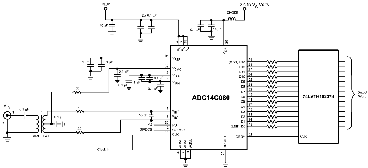
FIGURE 7. Application Circuit
